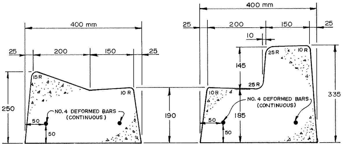
Residential Mountable Curb & Gutter
