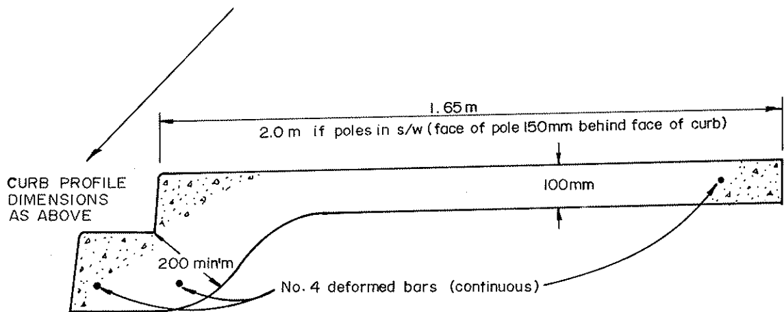
Combined Curb, Gutter & Sidewalk (MONOLITHIC)
