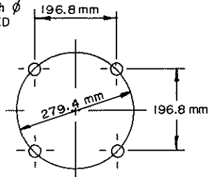
ANCHOR BOLT SPACING
