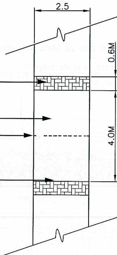
SIDEWALK PAVING DETAIL 1:100
