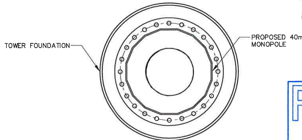
3 BASE PLAN VIEW
