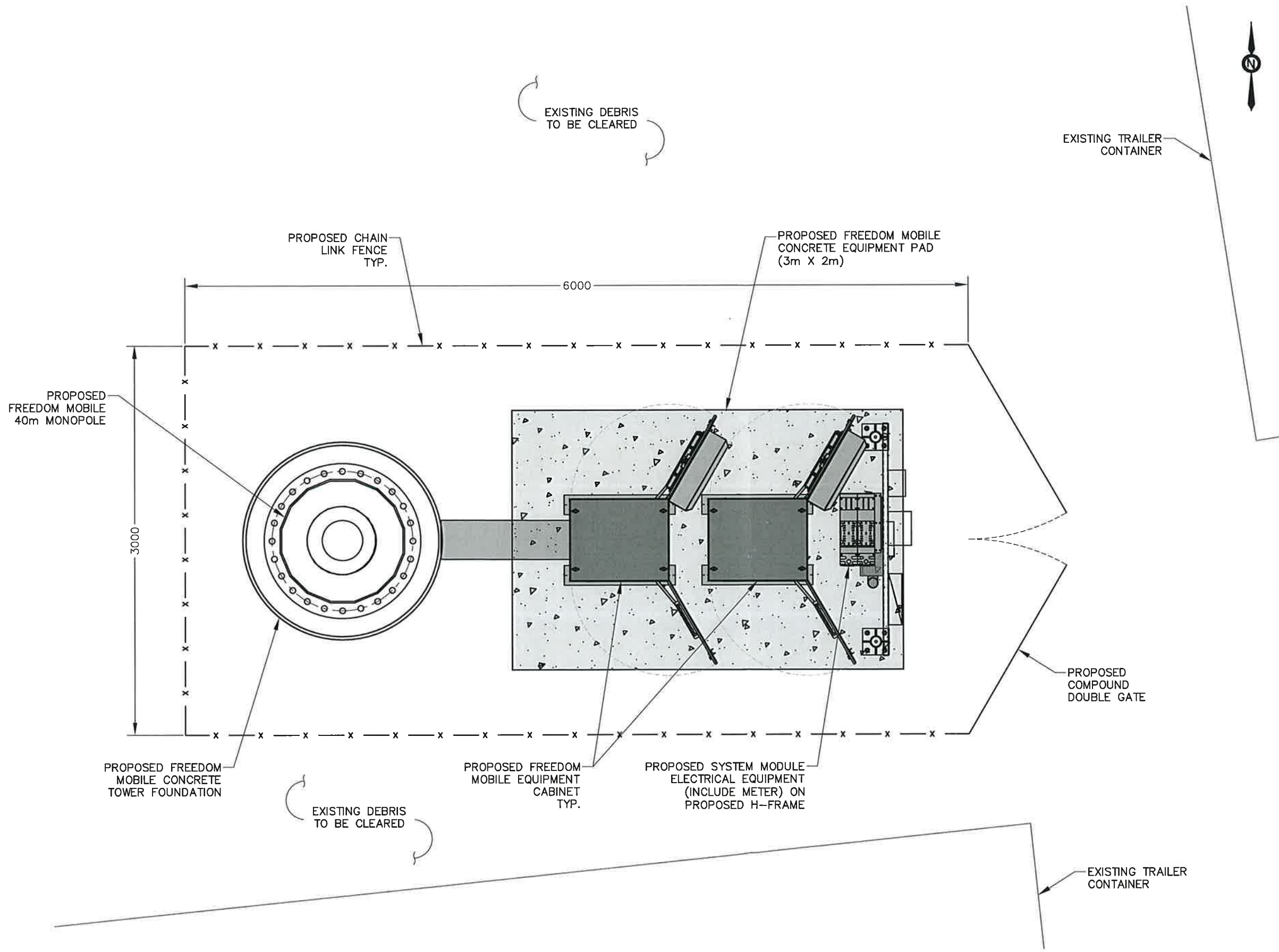
① COMPOUND LAYOUT
