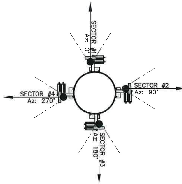
2 ANTENNA LAYOUT
